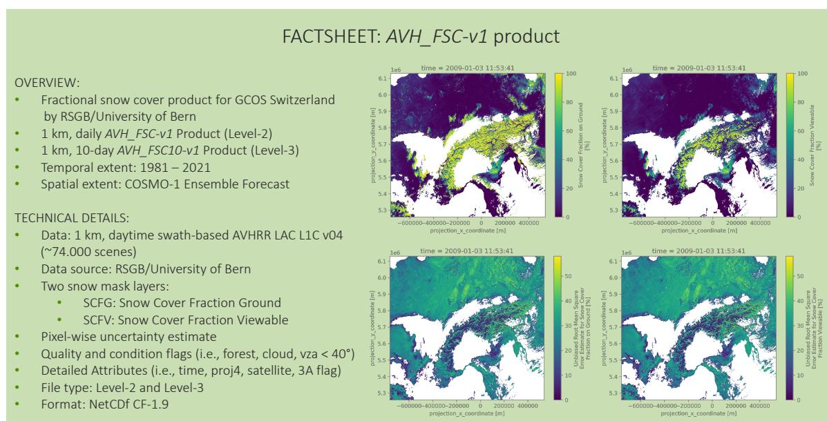
Figure 2: Factsheet of the AVH_FSC-v1 and AVH_FSC10-v1 product describing an overview and technical details of the novel fractional snow cover product. The example images of NOAA-18 (dated: 2009-01-03 11:53) show the SCFG (upper left) and SCFV (upper right) snow maps as well as their uncertainty estimations (SCFG: lower left), SCFV (lower right) for the COSMO-1E extent.
