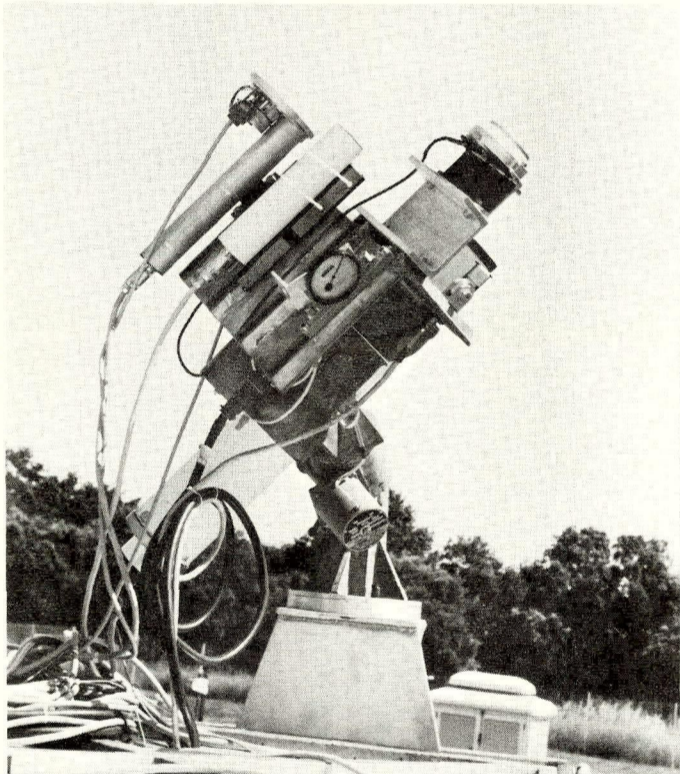
5. Side-view of the sun-tracking devices
