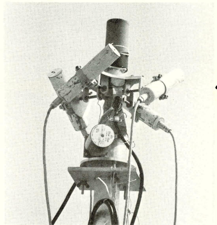
6. Four pyroelectric detectors scan the sky ( 5^{\circ} aperture) in 121 points in about 2 minutes
