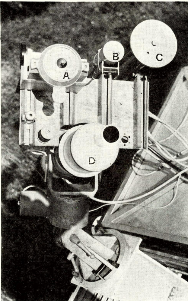
4. On the car's roof four instruments are mounted on an automatic sun-tracker: pyranometer (A), pyroelectric detector (B), absolute radiometer (C) with broad band Schott-filters OG1, RG2 and RGB and spectroradiometer (D) measuring at 16 different wavelengths
