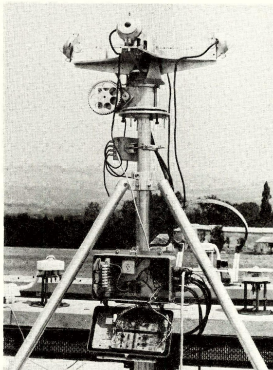
5. Side-view of the sun-tracking devices
