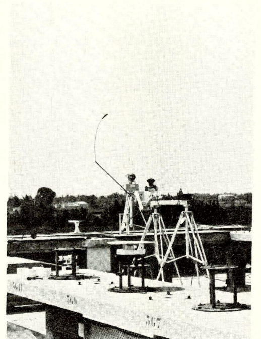
9. A shading disc always occults direct solar beam from a fish-eye camera
