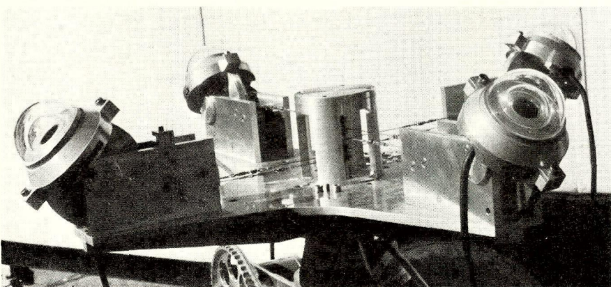
7. and 8. Four pyranometers are driven by step motors and measure in 77 different tilts and directions in about 6 minutes
